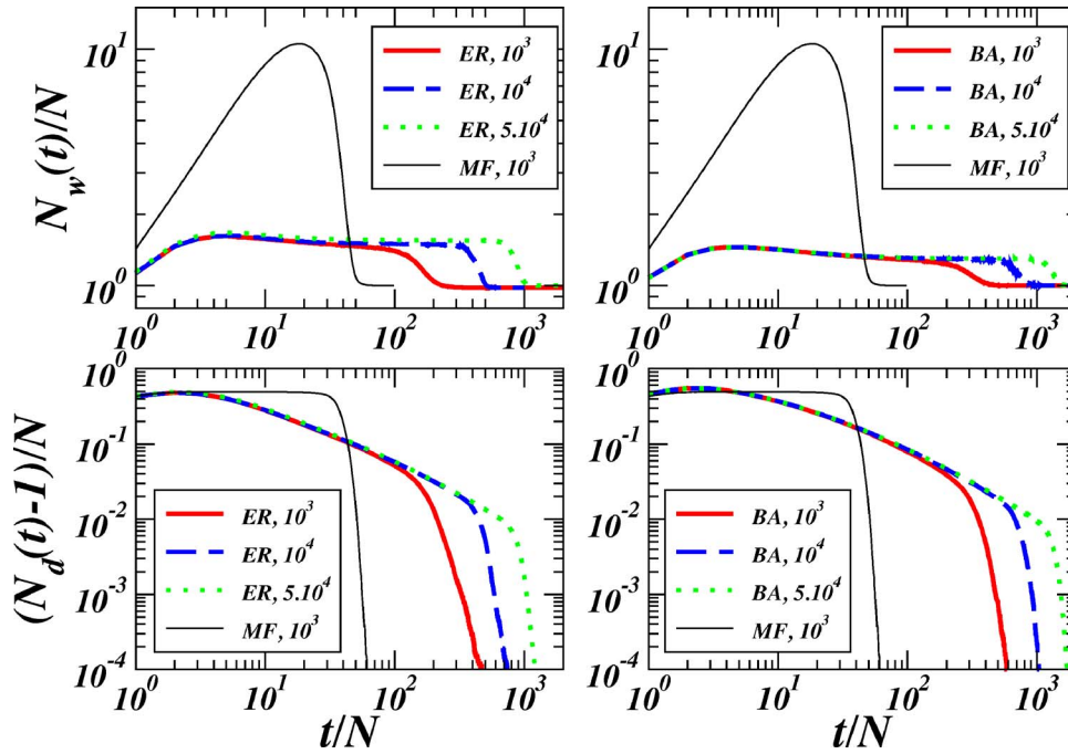
FIG. 5. ER random graph (left) and BA scale-free network (right) with \langle k \rangle = 4 and sizes N = 10^3, 10^4, 5 \times 10^4 . (Top) Evolution of the average memory per agent N_w/N vs rescaled time t/N . For increasing sizes a plateau develops in the reorganization phase preceding the convergence. The height of the peak and of the plateau collapses in this plot, showing that the total memory used scales with N . (Bottom) Evolution of the number of different words N_d in the system. (N_d - 1)/N is plotted in order to emphasize the convergence to the consensus with N_d = 1 . A steady decrease is observed even if the memory N_w displays a plateau. The mean-field (MF) case is also shown (for N = 10^3 ) for comparison.
