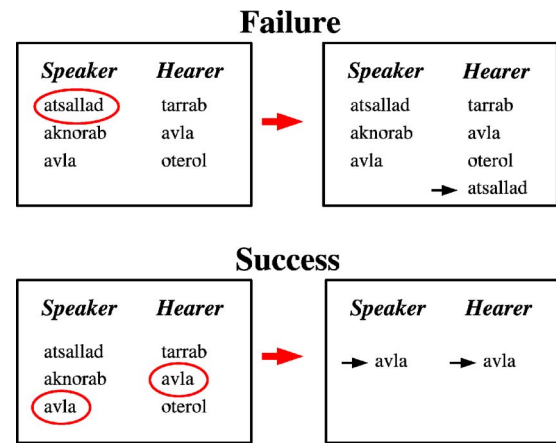
FIG. 1. Agent interaction rules. Each agent is described by its inventory, i.e., the repertoire of known words. The speaker picks up at random a name in its inventory and transmits it to the hearer. If the hearer does not know the selected word the interaction is a failure (top), and it adds the new name to its inventory. Otherwise (bottom), the interaction is a success and both agents delete all their words but the winning one. Note that if the speaker has an empty inventory (as it happens at the beginning of the game), it invents a new name and the interaction is a failure.
