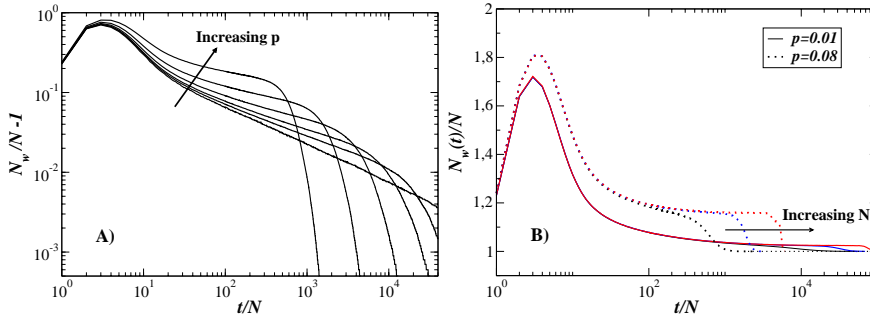
Fig. 1 – A) Average number of words per agent in the system, N_w/N , as a function of the rescaled time, t/N , for small-world networks with \langle k \rangle = 8 and N = 10^3 nodes, for various values of p . The curve for p = 0 is shown for reference, as well as p = 5 \cdot 10^{-3} , p = 10^{-2} , p = 2 \cdot 10^{-2} , p = 4 \cdot 10^{-2} , p = 8 \cdot 10^{-2} , from bottom to top on the left part of the curves. B) (Color on-line) N_w/N for p = 10^{-2} and p = 8 \cdot 10^{-2} and increasing system sizes: N = 10^3 , N = 10^4 , N = 10^5 . Larger system sizes yield larger plateau lengths.
