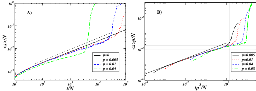
Fig. 4 – (Color on-line) A) Evolution of the cluster size for N = 10^4 , various values of p . At increasing p the curves depart more and more from the t^{1/2} behavior through a slowing down of the cluster growth, which however leads to a faster convergence. B) Same curves rescaled around the crossover region.
