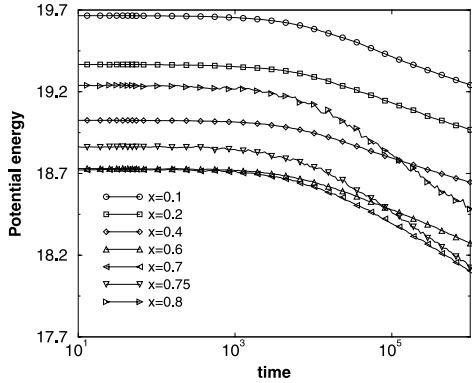
Figure 5. Potential energy (or mean height) of the system, for various x and measured after t_w = 10^4 .
