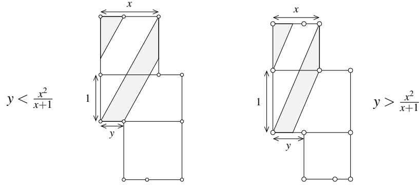
FIGURE 8. Cylinders in direction \theta_3 of slope \frac{x+1}{x} when t = 0 . If y \neq \frac{x^2}{x+1} then there always exists a simple cylinder in direction \theta_3 .
