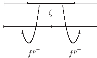
FIGURE 3. Doubly returning, doubly periodic \zeta (no switches)
