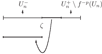
FIGURE 6. Q_p = U_n^- \cup (U_n^+ \setminus f^{-p}(U_n))
